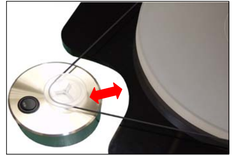
Picture 5: Placing the motor
