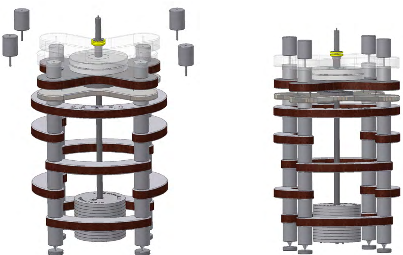
Pic. 18: Setting the arm bases
