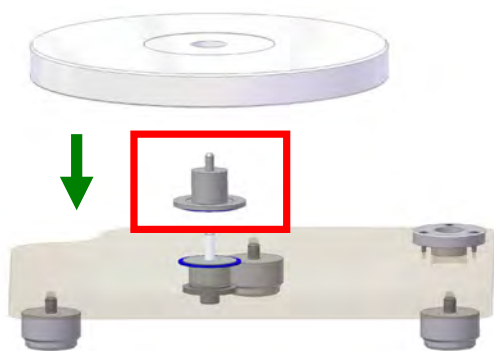
Pic. 3: Placing the bearing
