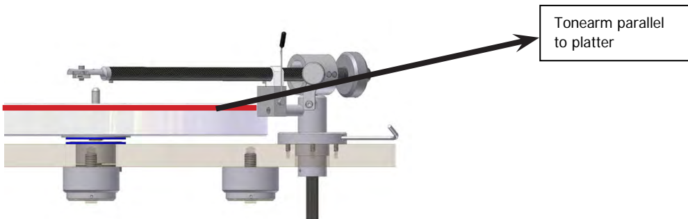
Pic. 9: Setting the VTA
