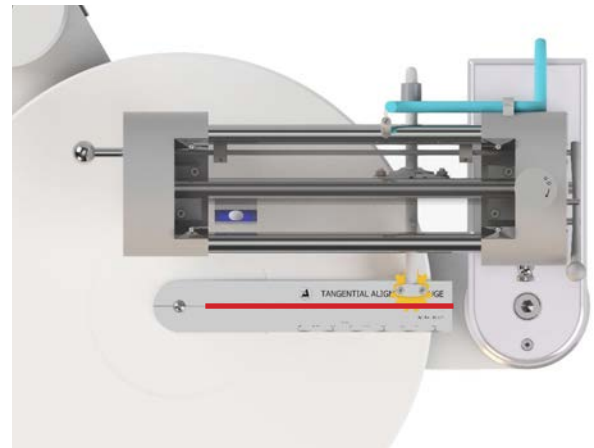
Pic. 26a: Adjustment of the linear tracking
