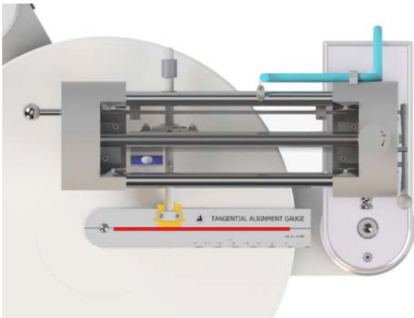
Pic. 26: Adjustment of the linear tracking
