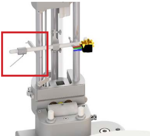
Pic. 21: Fixing the counterweight
