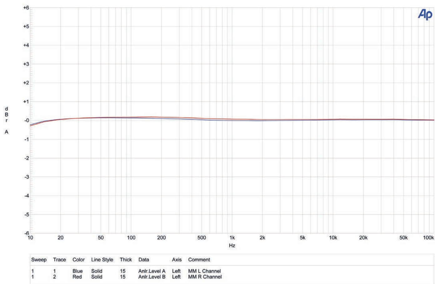
Pic. 5: Frequency Response
