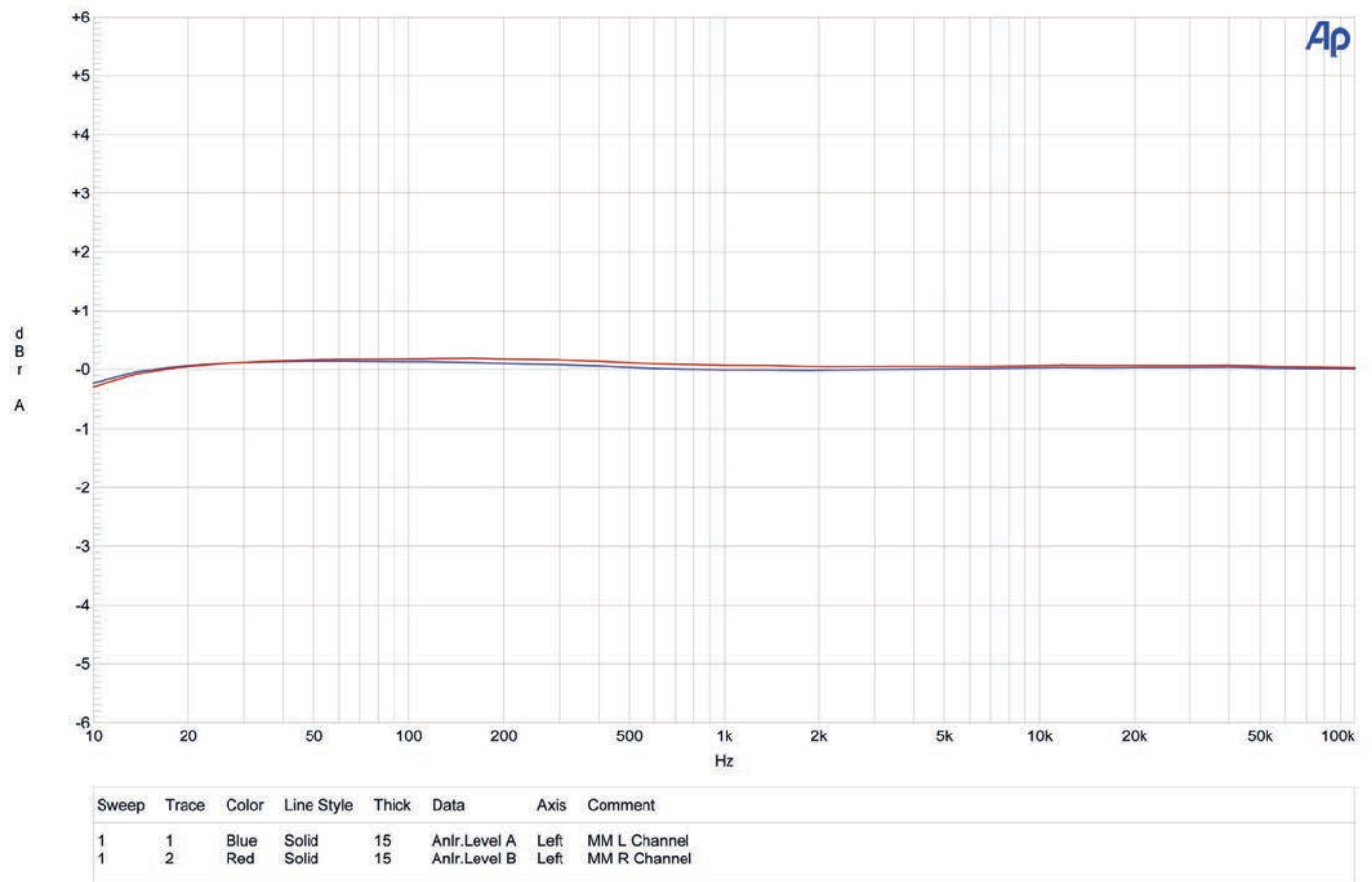
Abb. 5: Frequenzgang
