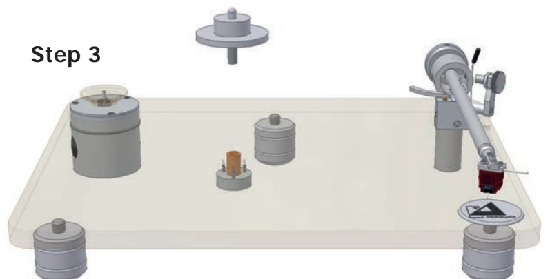
Picture 3: Taking off the standard bearing
