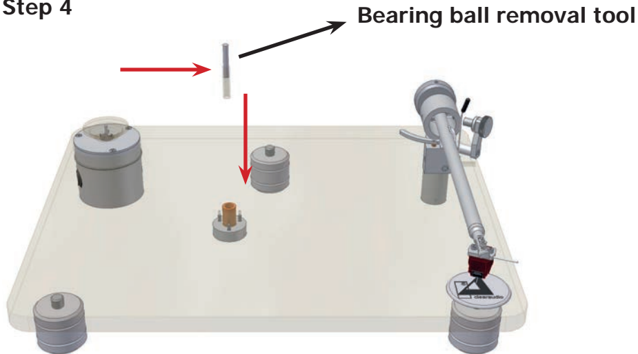
Picture 4: Removing the bearing ball. Please use the tool to remove the bearing ball.
