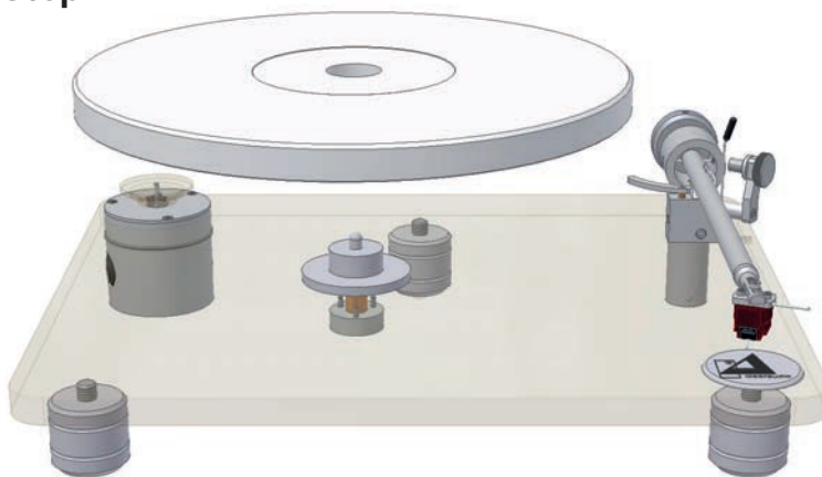
Picture 2: Taking off the platter
