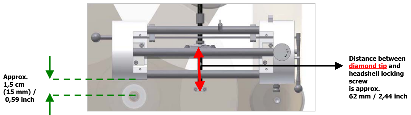
Pic.10: Correct position of the headshell
