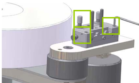
Pic.3: Tighten the three screws of the tonearm
