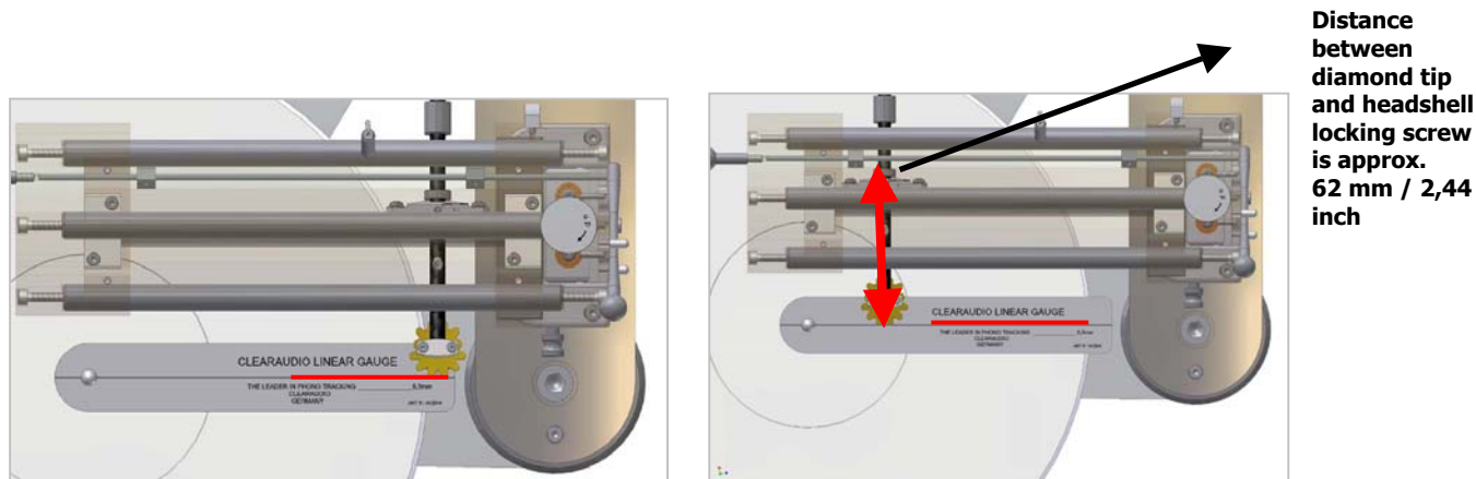
Pic.17: Adjustment of the linear tracking
