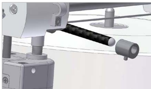
Pic.12: Set up of counterweight(s)
