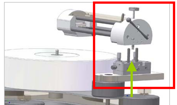
Pic.5: Placing the tonearm on the tonearm base
