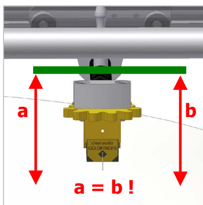
Pic.16: Adjustment of the Azimuth
